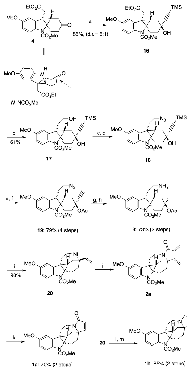
Scheme 3. Total synthesis of 1a and 1b .
